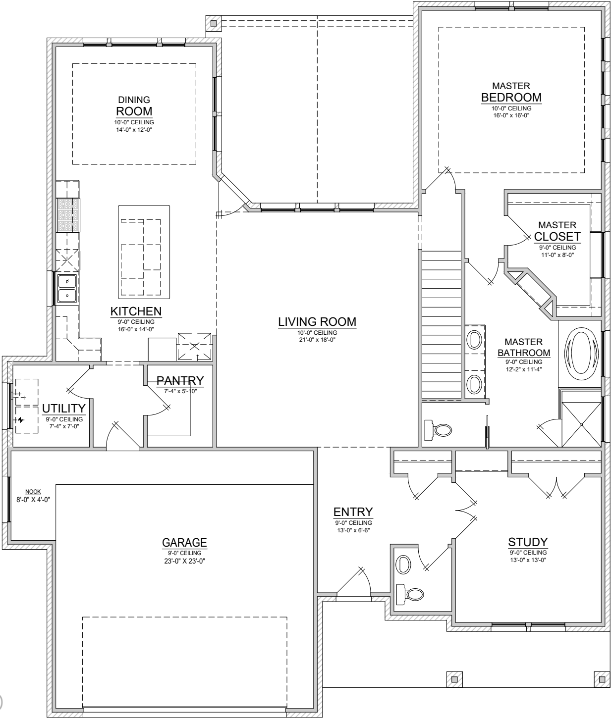
FIRST FLOOR PLAN 2,005 SQ. FT.
