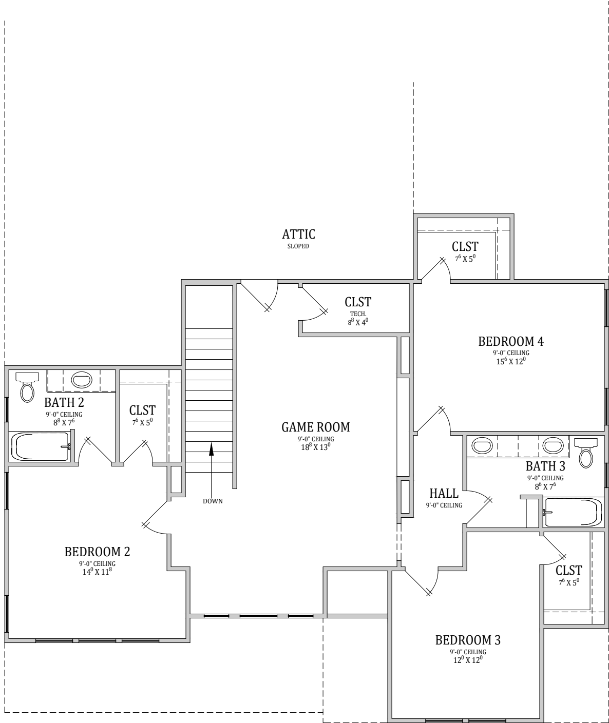
SECOND FLOOR PLAN 1,346 SQ. FT.
